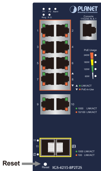
Figure 6-1: IGS-4215 PoE Series Reset Button
